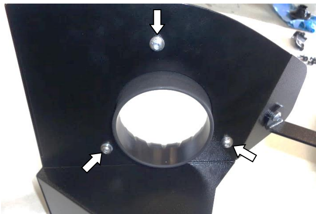
21. Assemble air filter adapter (3) to heat shield using M6 screws (6), lock washers (5) and flat washers (4).
