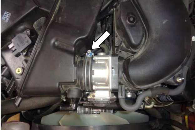
13. Loosen the hose clamp securing the airbox to the throttle body.
