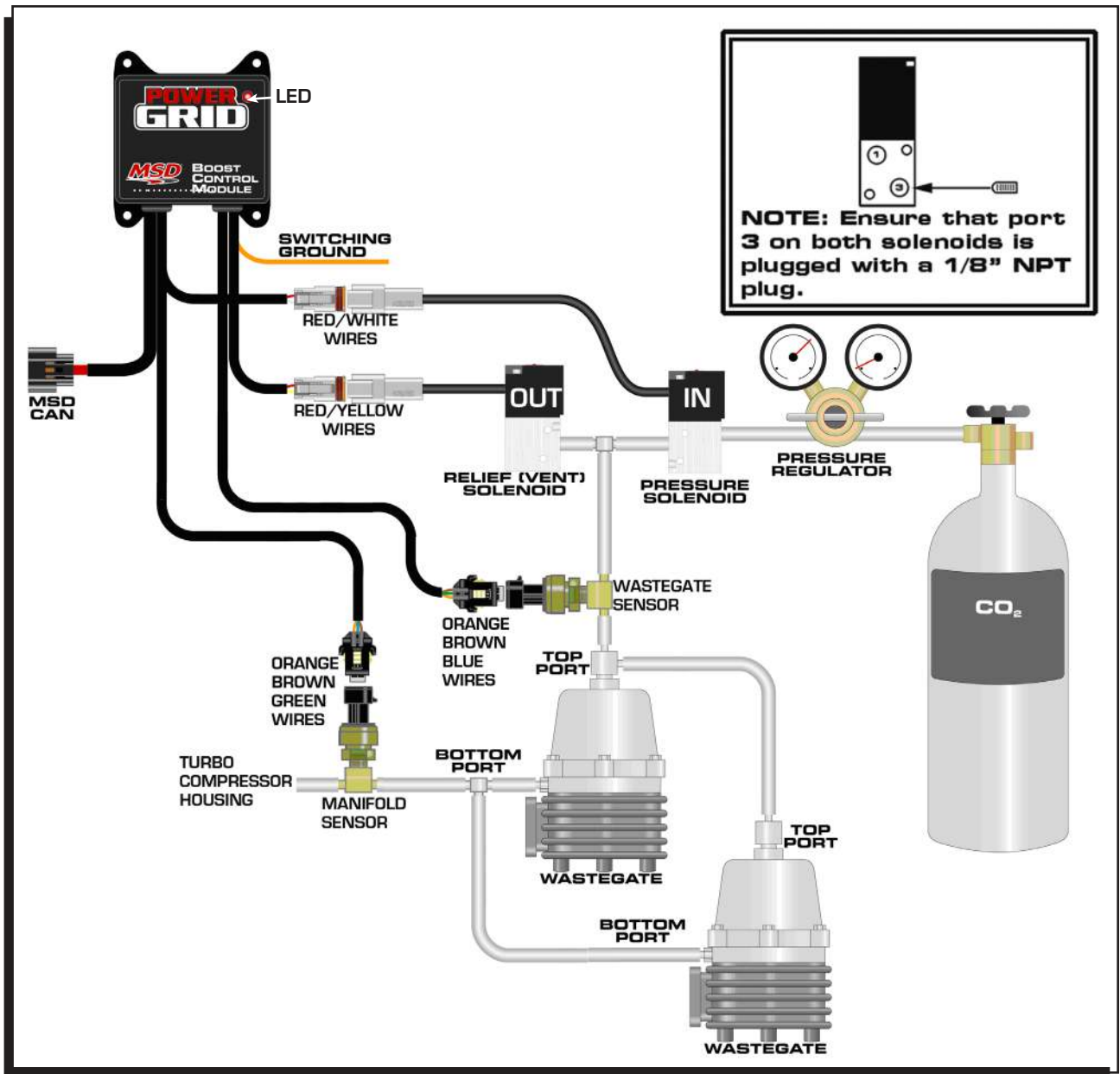
Figure 2 Dual Wastegate Plumbing
