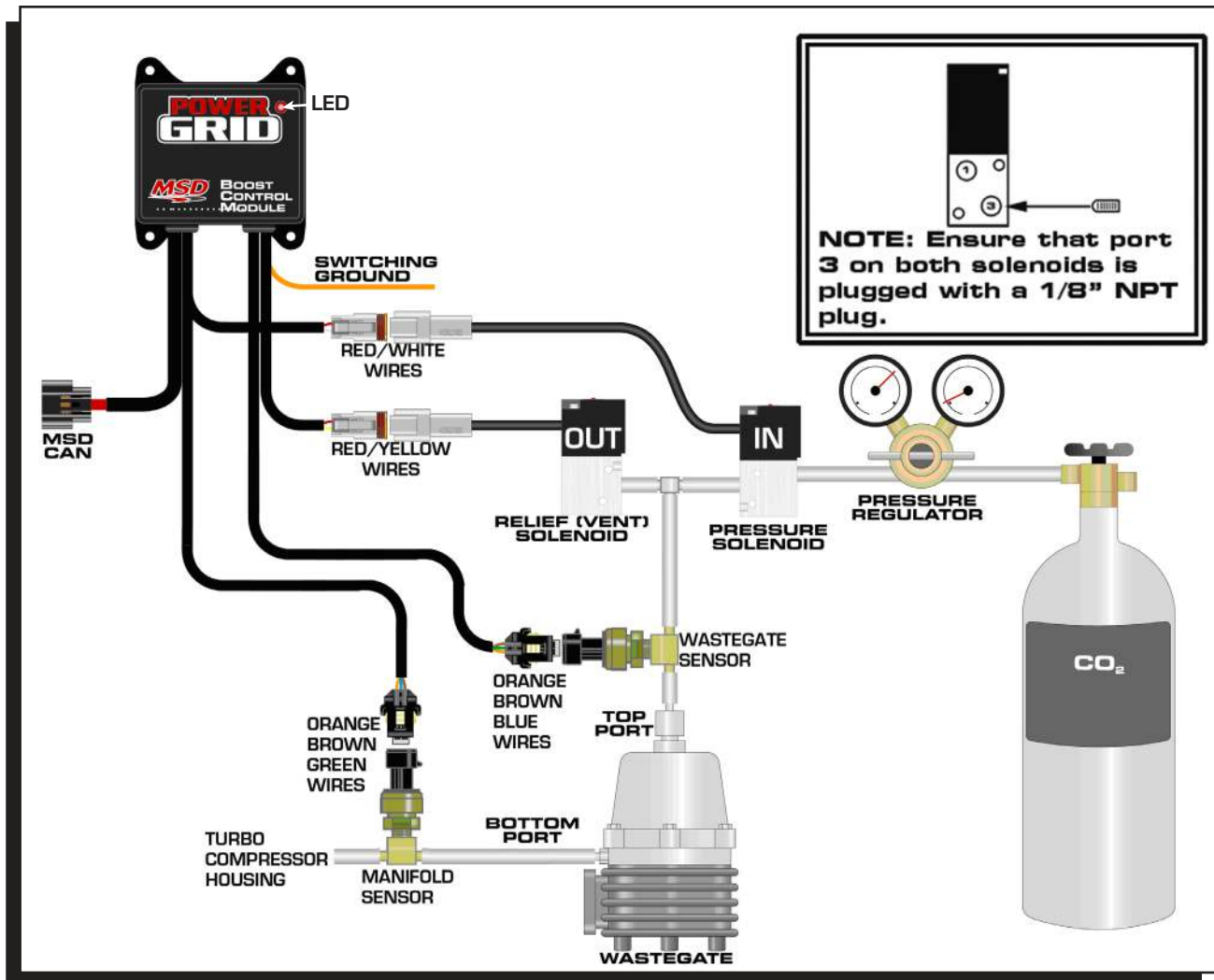
Figure 1 Single Wastegate Plumbing
