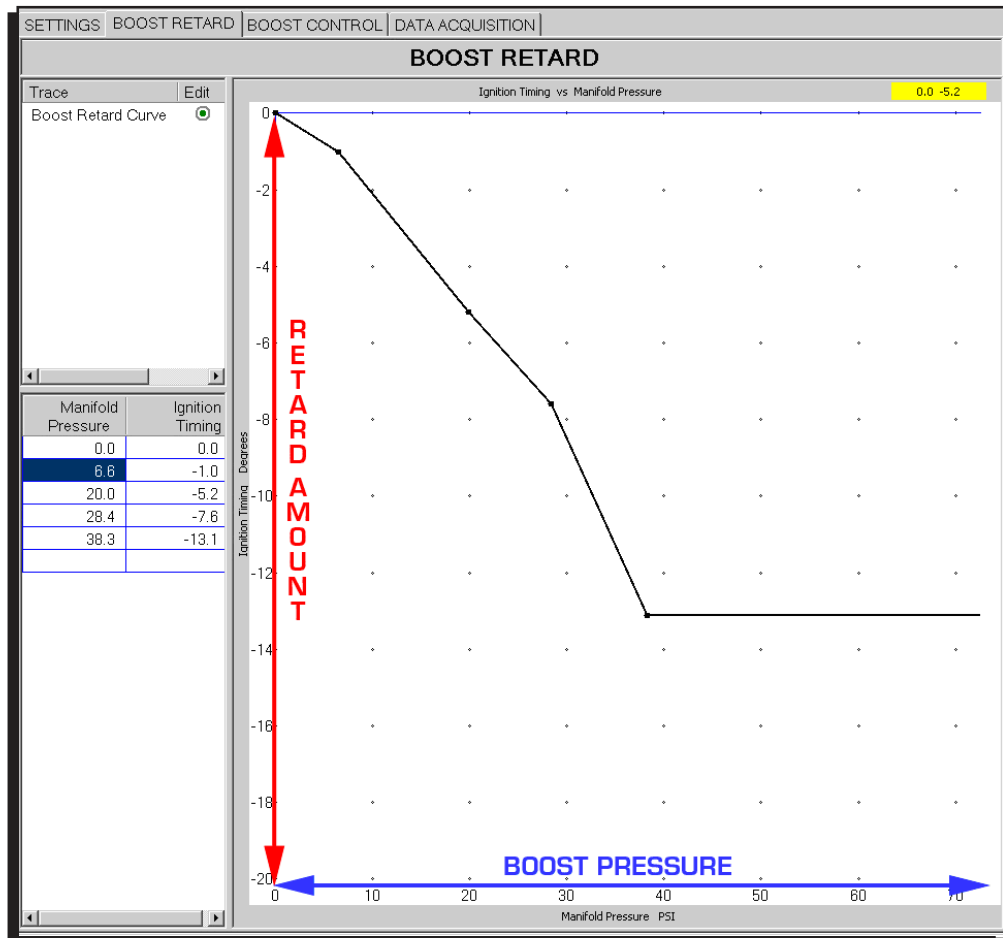
Figure 6 Boost Retard
