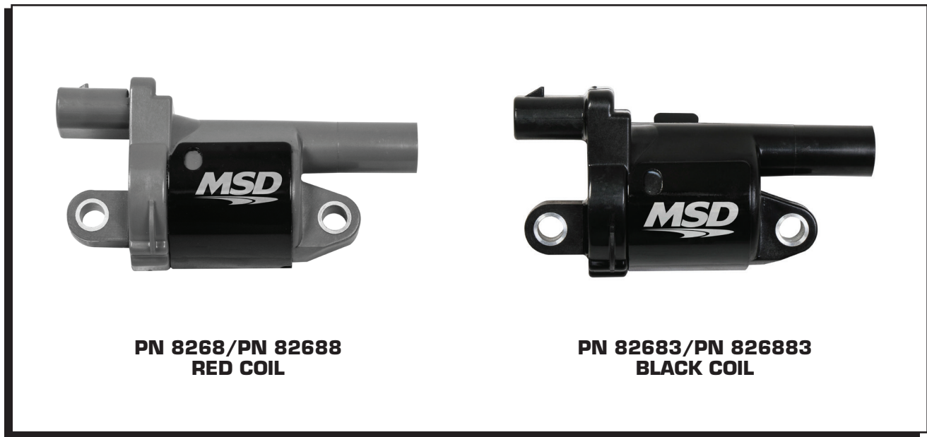
Figure 1 Coils
